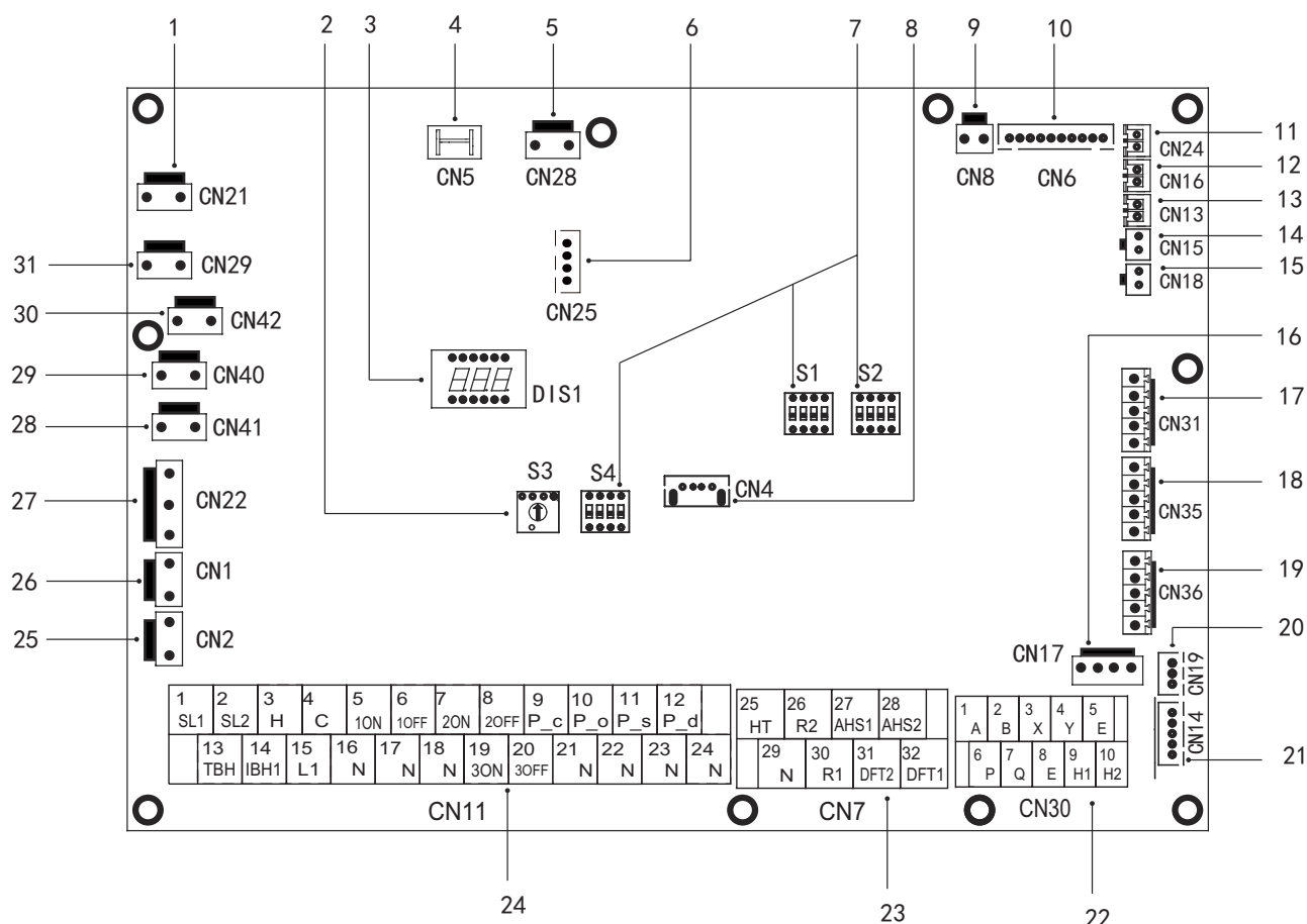
fig. 23 - Hydronic board
